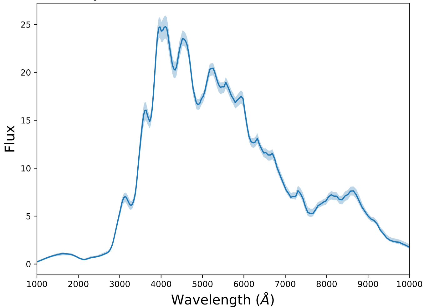
Spectrum 5 for transient SNIax at z=0.90
